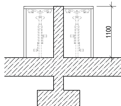
SECTION SCALE 1:50
