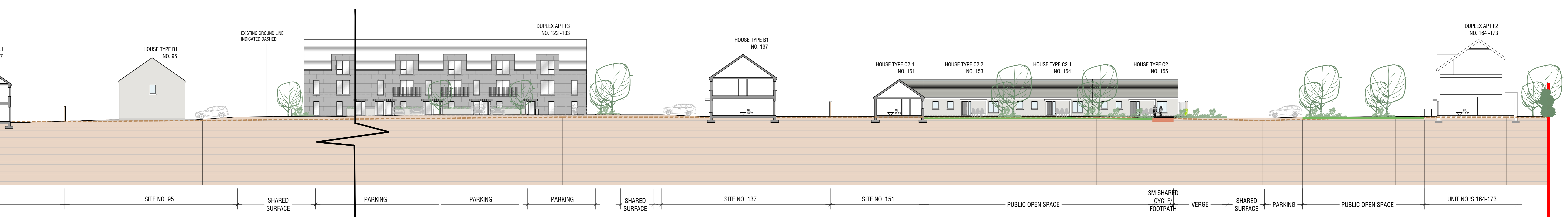
SITE SECTION E-E - CONTIGUOUS ELEVATION (cont.) SCALE 1:200
