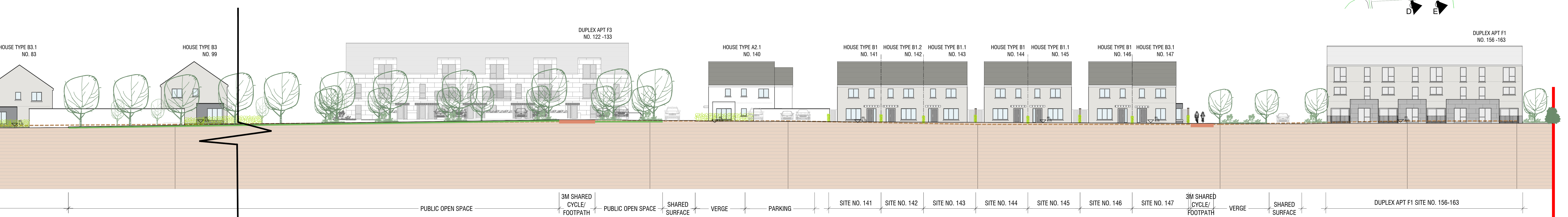
SITE SECTION D-D - CONTIGUOUS ELEVATION (cont.) SCALE 1:200
