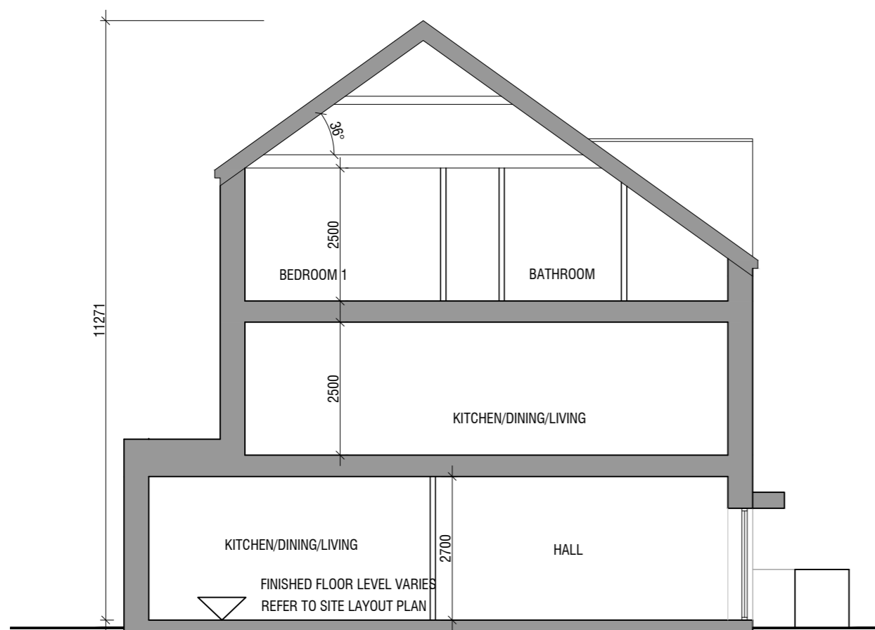
F3 TYPICAL SECTION 1:100
