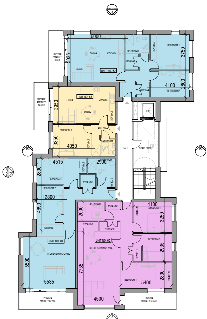
E2 FIRST FLOOR LEVEL SCALE 1:200
